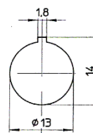
Mounting holes
